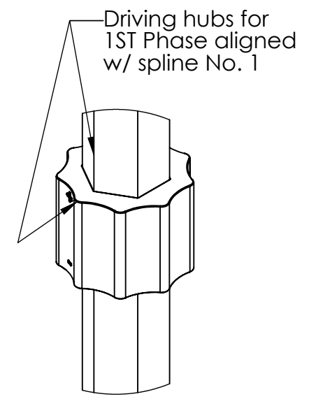
DETAIL F SCALE 1 : 3
