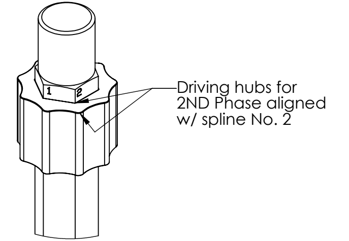
DETAIL E SCALE 1 : 3
